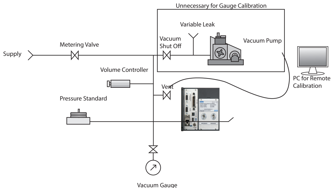
Figure 10.4 - Calibration Setup
